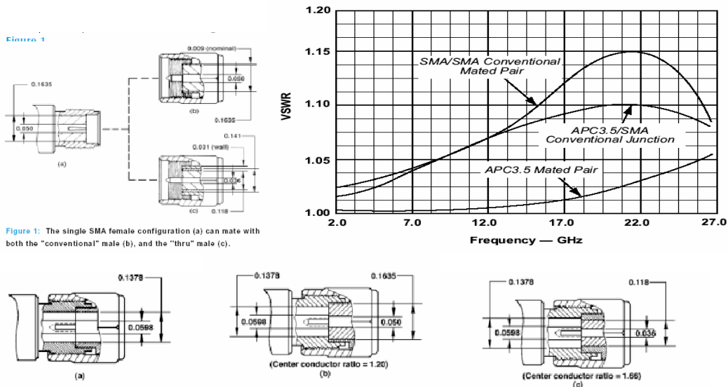
Figure 3: An APC3.5 mated pair (a) provides a precision junction with no discontinuities. Line size discontinuities are apparent when the APC3.5 mates to a "conventional" SMA connector (b), and are more of a problem with the SMA "thru" male (c).
