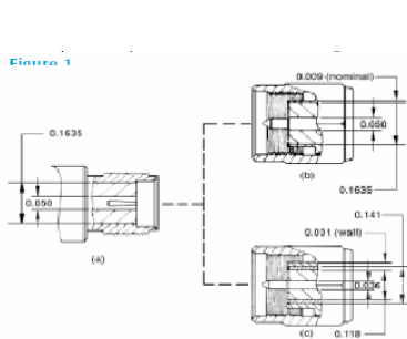
Figure 1: The single SMA female configuration (a) can mate with both the "conventional" male (b), and the "thru" male (c).
