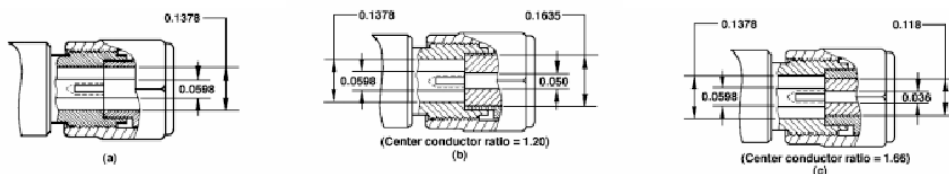
Figure 3: An APC3.5 mated pair (a) provides a precision junction with no discontinuities. Line size discontinuities are apparent when the APC3.5 mates to a "conventional" SMA connector (b), and are more of a problem with the SMA "thru" male (c).
