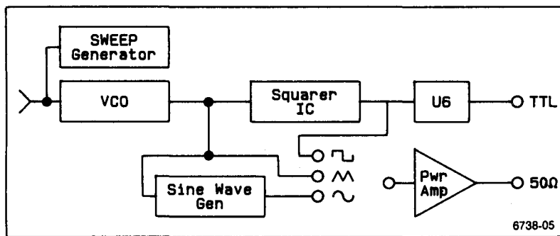
Figure 5-1. Circuit Block Diagram.
