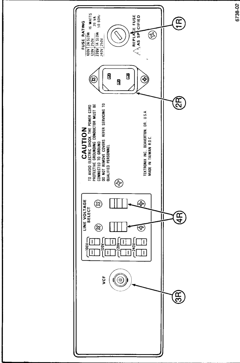
Figure 2-2. Rear Panel.
